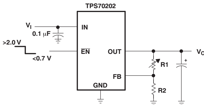
Figure 40. TPS70202 Adjustable LDO Regulator Programming
